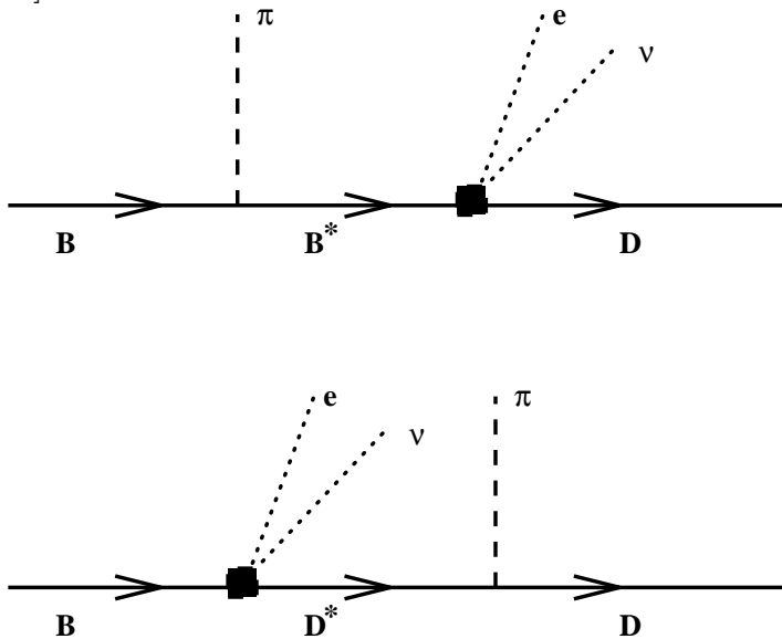
Figure 10 Feynman diagrams for B \rightarrow D e \nu
