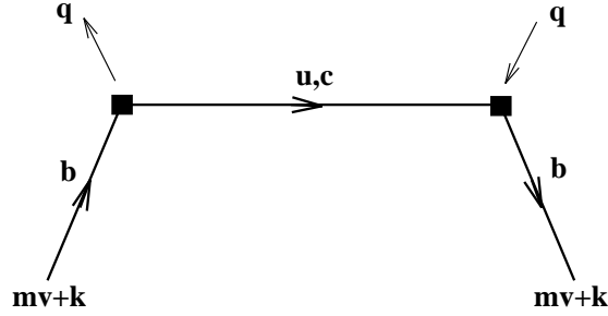
Figure 8 Tree level Green function for the product of currents.
