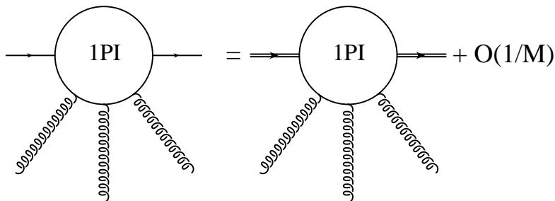
Figure 1 Relation between Green functions in full and effective field theories.
