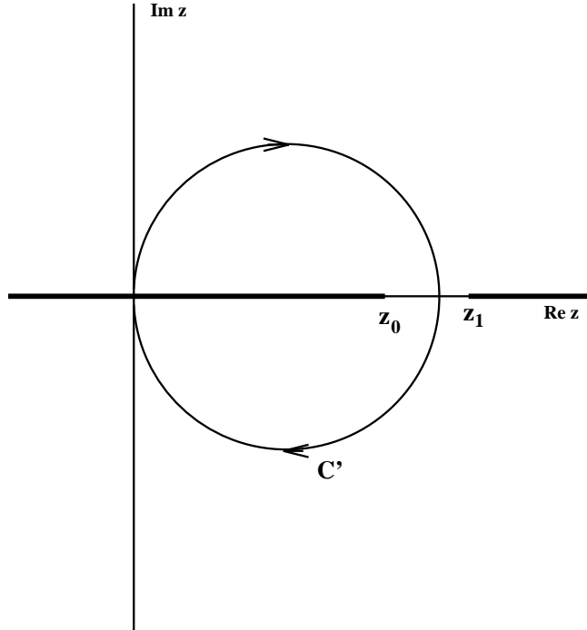
Figure 7 Deformed contour of integration, C' , in the dispersion relation (5.8). Note that it stays away from the physical region everywhere except near z=0 , provided Z_0 and z_1 are well separated.
