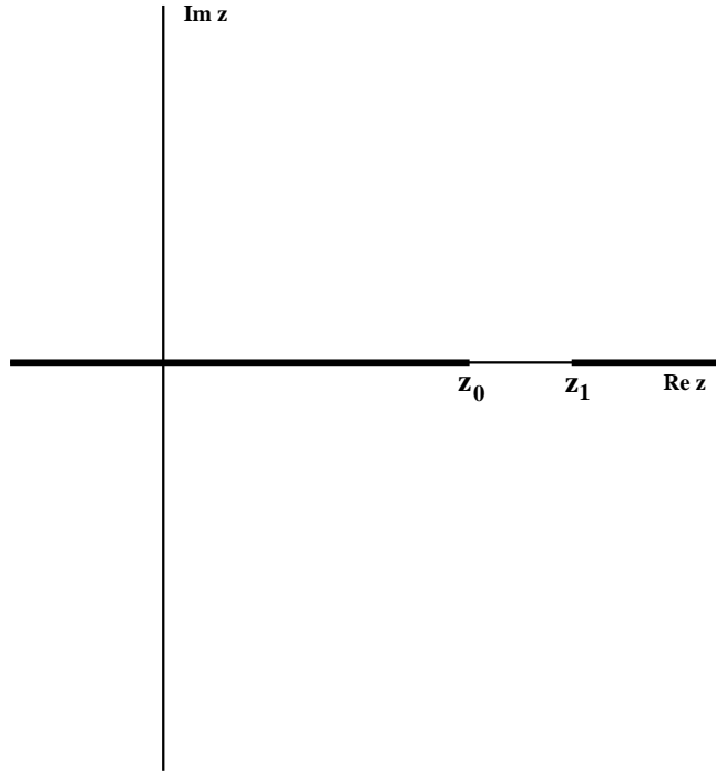
Figure 5 The location of the cuts in the complex z -plane.
