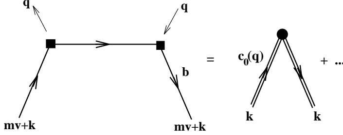
Figure 9 Representation of the combined OPE-HQET at tree level.
