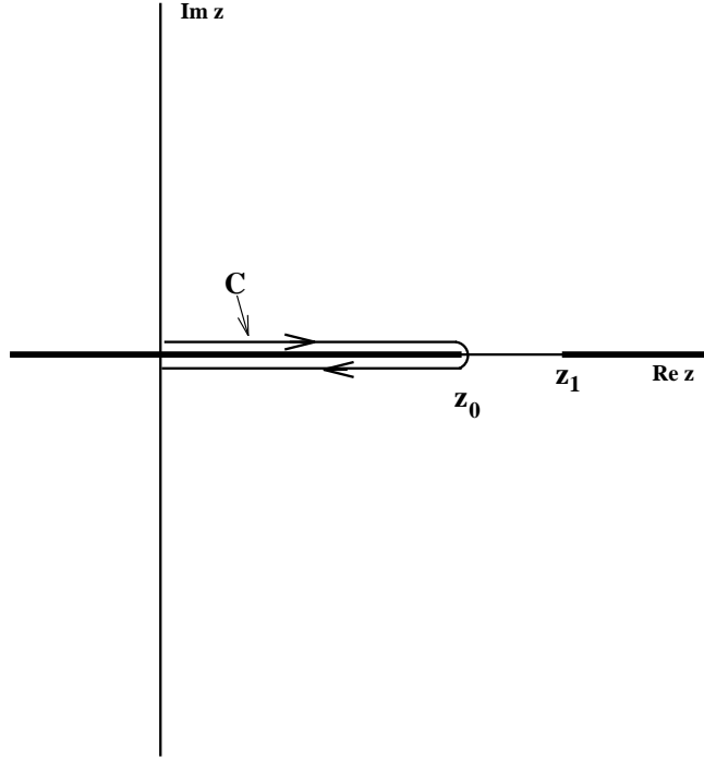
Figure 6 Contour of integration, C , in the dispersion relation (5.8).
