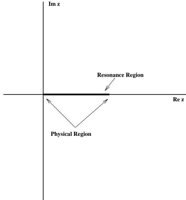
Figure 4 The location of the physical and resonant regions in the complex z -plane. The variable z is the energy of the final hadronic system in the semileptonic B decay, in the B restframe.
