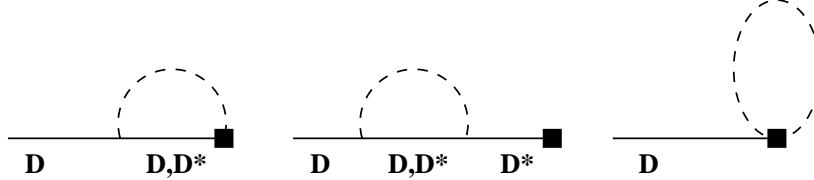
Figure 11 Feynman Diagrams in the calculation of f_{D_s}/f_D .
