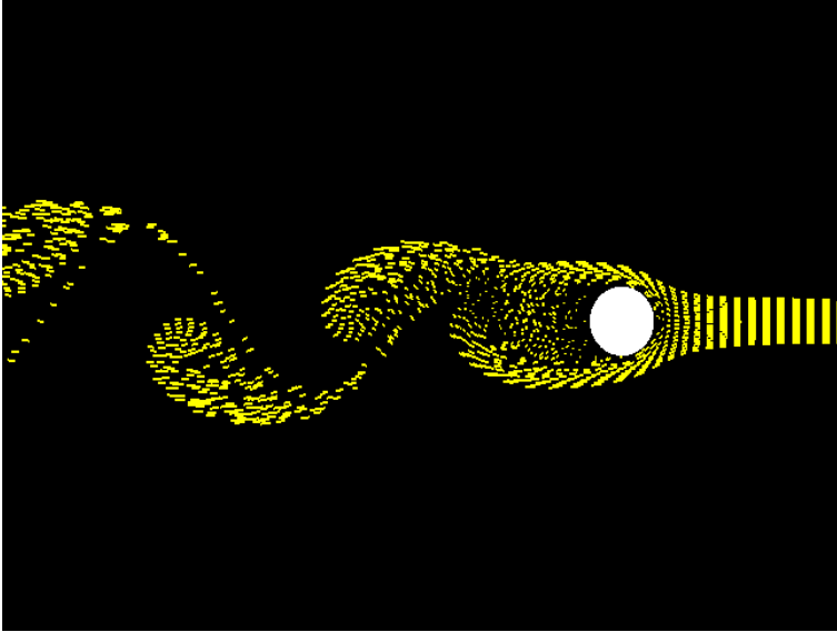
Simulation of fluid flowing around a sphere. "Drag of a Sphere" by Glenn Research Center Learning Technologies Project, NASA, via GIPHY is in the Public Domain, CCO
