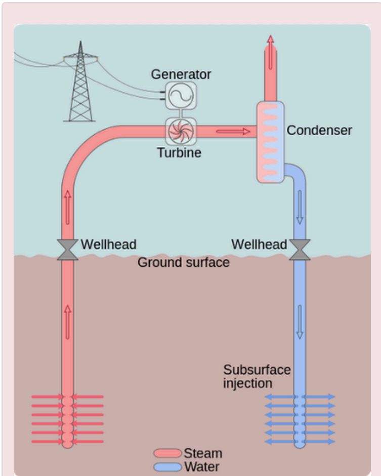
The dry steam cycle from "Geothermal power plants" by Energy Education, University of Calgary
