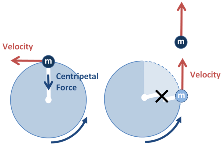
Left: A ball on a string undergoing circular motion with uniform (constant) speed. Right: The ball's trajectory after the string breaks. Image Credit: Breaking String by Brews ohare via Wikimedia Common
