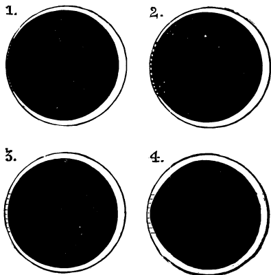
FIG. 9.—"Baily's Beads," four stages, at brief intervals. May 15, 1836.
