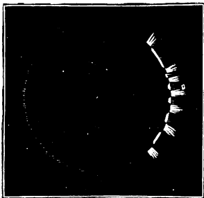
FIG. 8.—Brushes of light.
