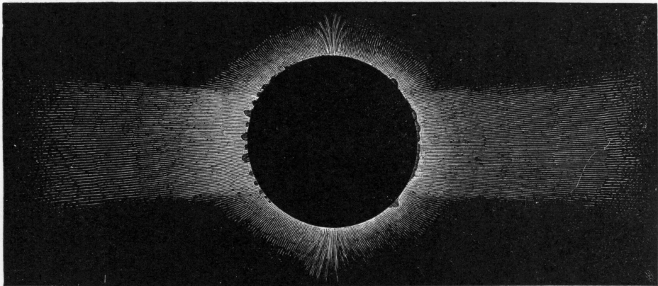
FIG. II.—Corona of 1867. (Sun-spot minimum.)
