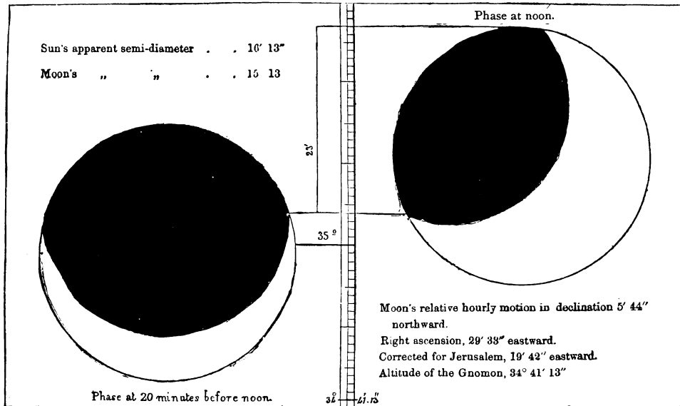
FIG. 12.—Solar eclipse at Jerusalem, 11th January, B. C. 680.
