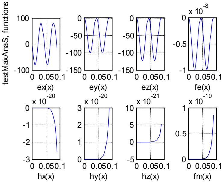
Fig. 9.4.3a. Electrical charges in vacuum
