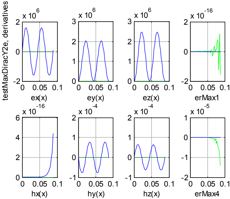
Fig. 9.3.3.2b. Electrical charges in vacuum.
