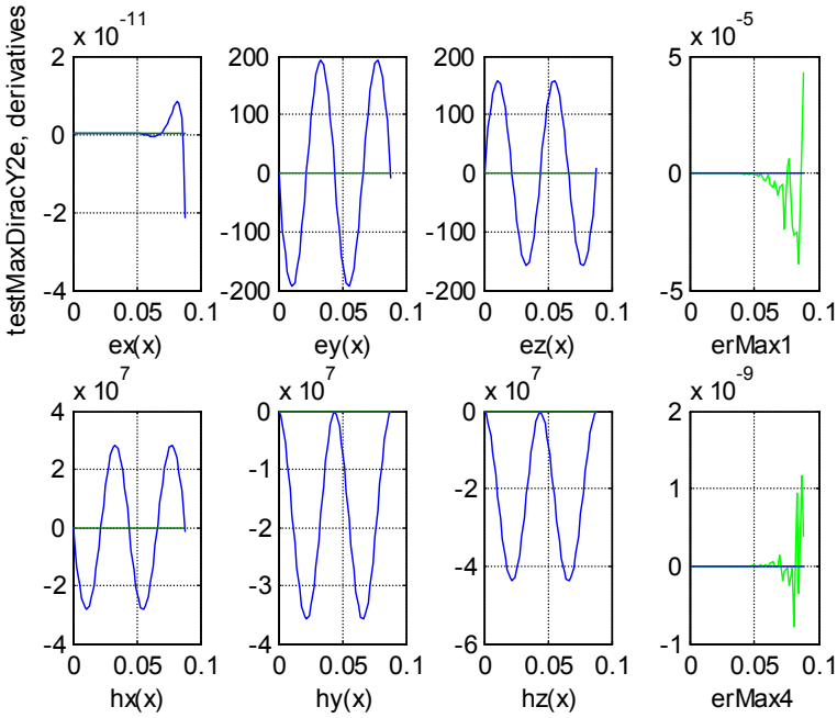
Fig. 9.3.3.1b. Magnetic charges in vacuum.
