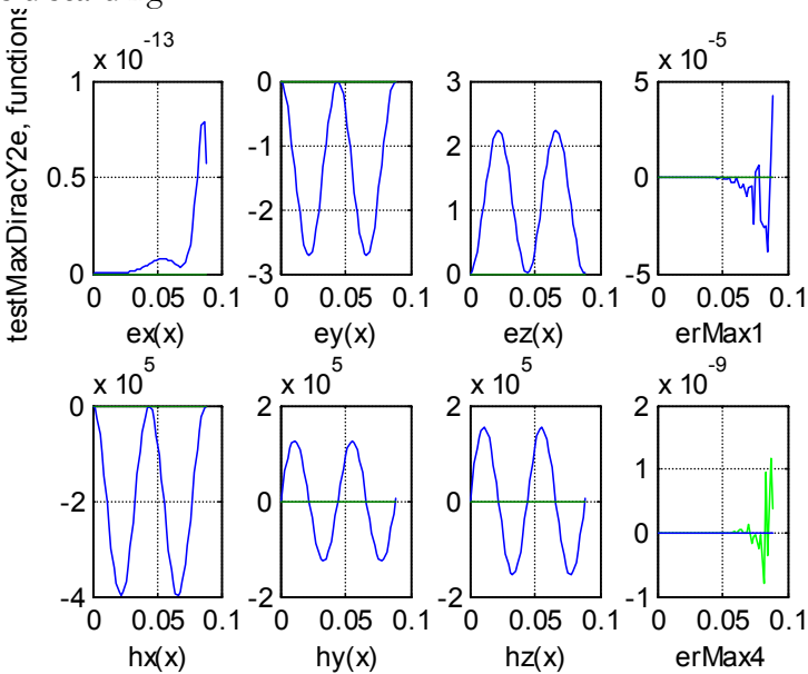
Fig.. 9.3.3.1a. Magnetic charges in vacuum.
