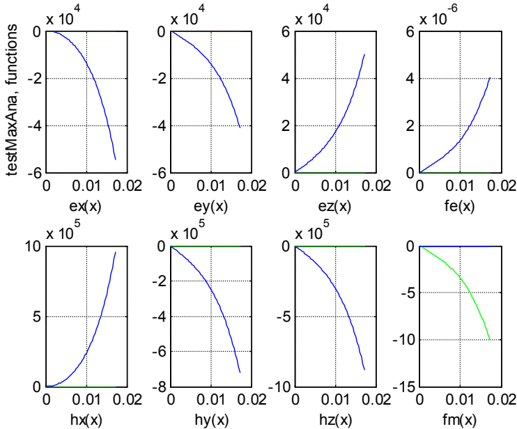
Fig. 9.5.1a. General solution for \Xi(x) = \lambda'(x) ,
