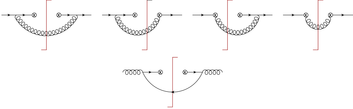
Figure 7.1. One-loop diagrams contributing to the matching coefficients \mathcal{I}_{q\leftarrow q} (top row) and \mathcal{I}_{q\leftarrow g} (bottom row). The vertical lines indicate cut propagators.
