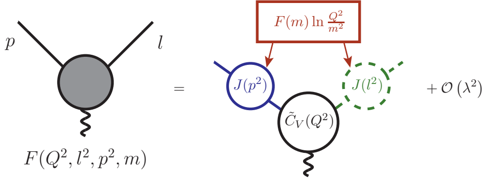
Figure 4.3. Diagrammatic representation of the Sudakov form factor in presence of a collinear anomaly; the diagram illustrates the separation of the different scales present in the problem, after re-factorization.
