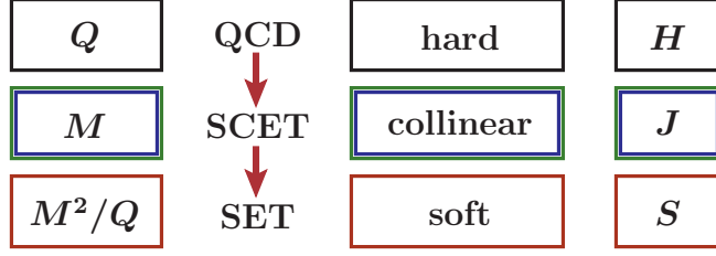
Figure 2.2. Chart of regions and scales involved in the calculation. Q indicates the hard scale, M the scale characterizing collinear physics, and M^2/Q the soft scale. SET stands for Soft Effective Theory.
