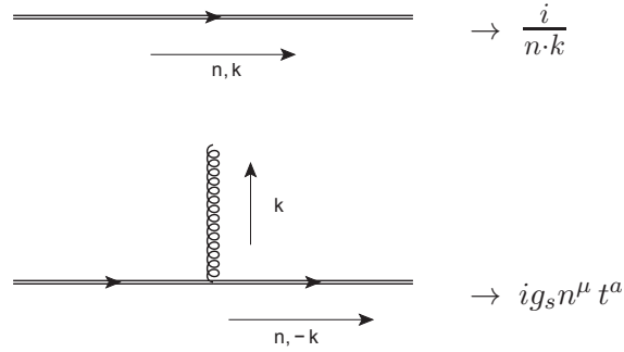
Figure E.2. Feynman rules derived from the Lagrangian for the field \phi .
