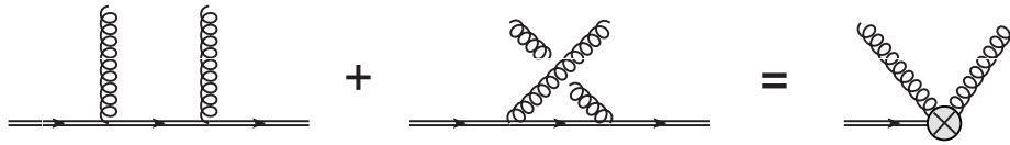
Figure E.2. Feynman rules derived from the Lagrangian for the field \phi .
