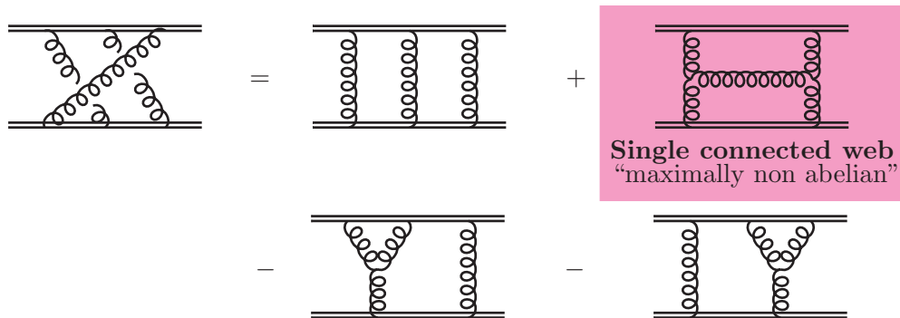
Figure 8.4. Decomposition of a web in a sum of products of connected webs.
