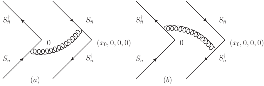
Figure B.1. Non-zero one-loop diagrams contributing to \hat{W}_{\text{DY}}(x, \mu) at order \alpha_s .
