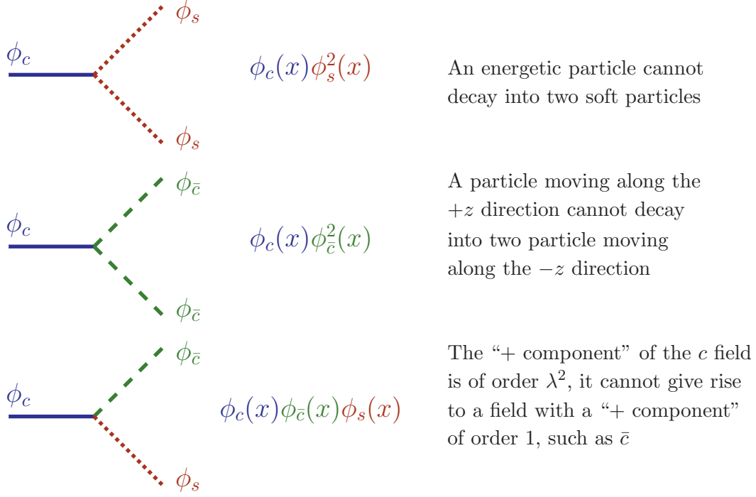
Figure 3.2. Interaction forbidden by momentum conservation.
