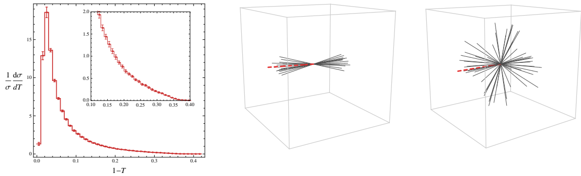
Figure 9.1. Left: The thrust distribution as measured by the ALEPH experiment at LEP I [226]. The inset shows the region relevant for the \alpha_s determination. Right: Sample collider events. The two-jet configuration on the left has a large thrust T \approx 0.98 , while the multi-jet event on the right has T \approx 0.65 (note that a completely spherical event has T = 1/2 ). The red dashed line indicated the thrust vector.
