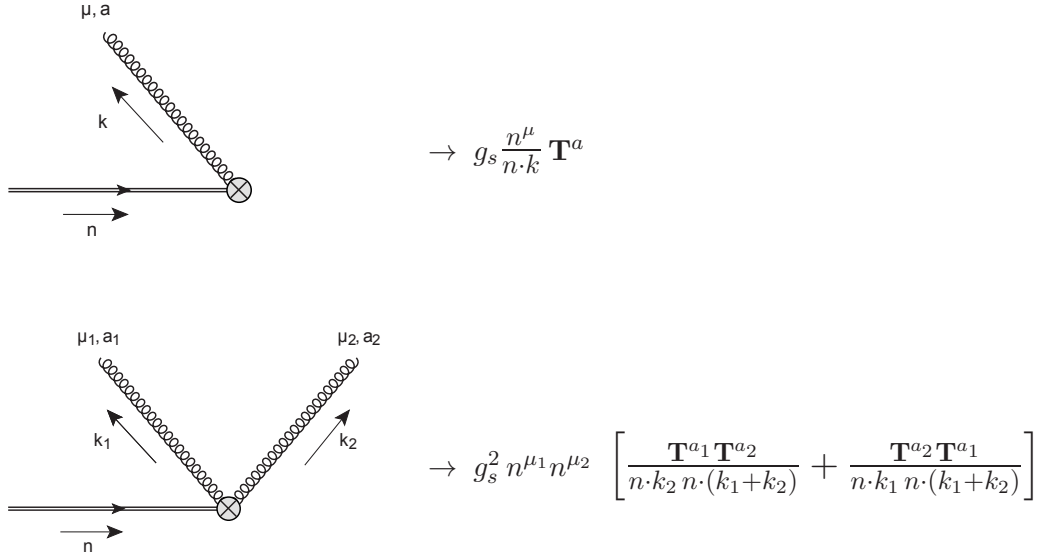
Figure E.1. Feynman rule for the emission of one and two gluons from a soft Wilson line.
