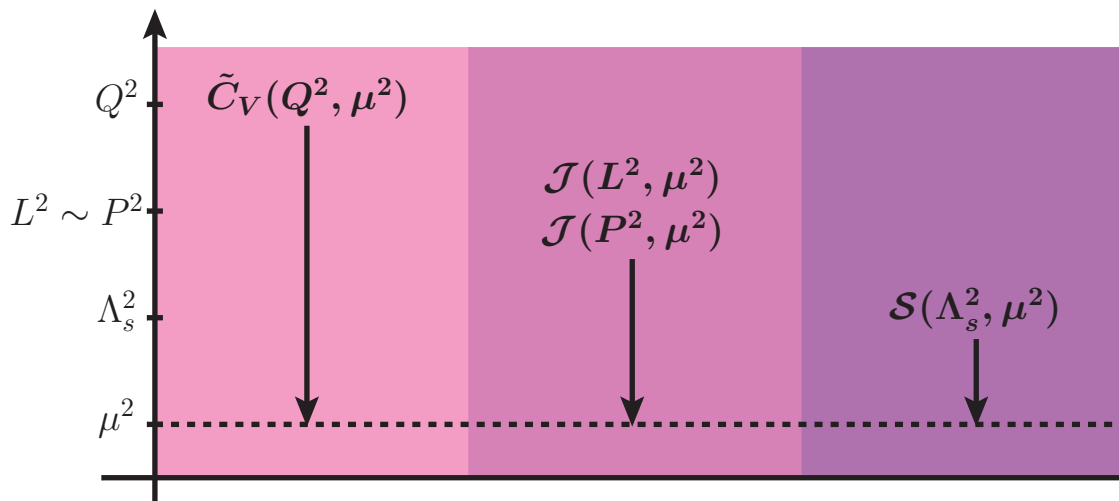
Figure 5.2. Schematic representation of the scale separation and of the calculational procedure in renormalization group improved perturbation theory.
