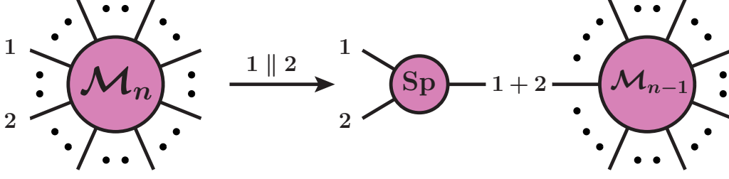
Figure 8.5. Schematic representation of the amplitude factorization in the collinear limit.
