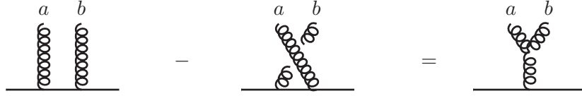
Figure 8.3. Diagrammatic form of the Lie commutator relation in the case in which the particle emitting soft radiation is a quark.
