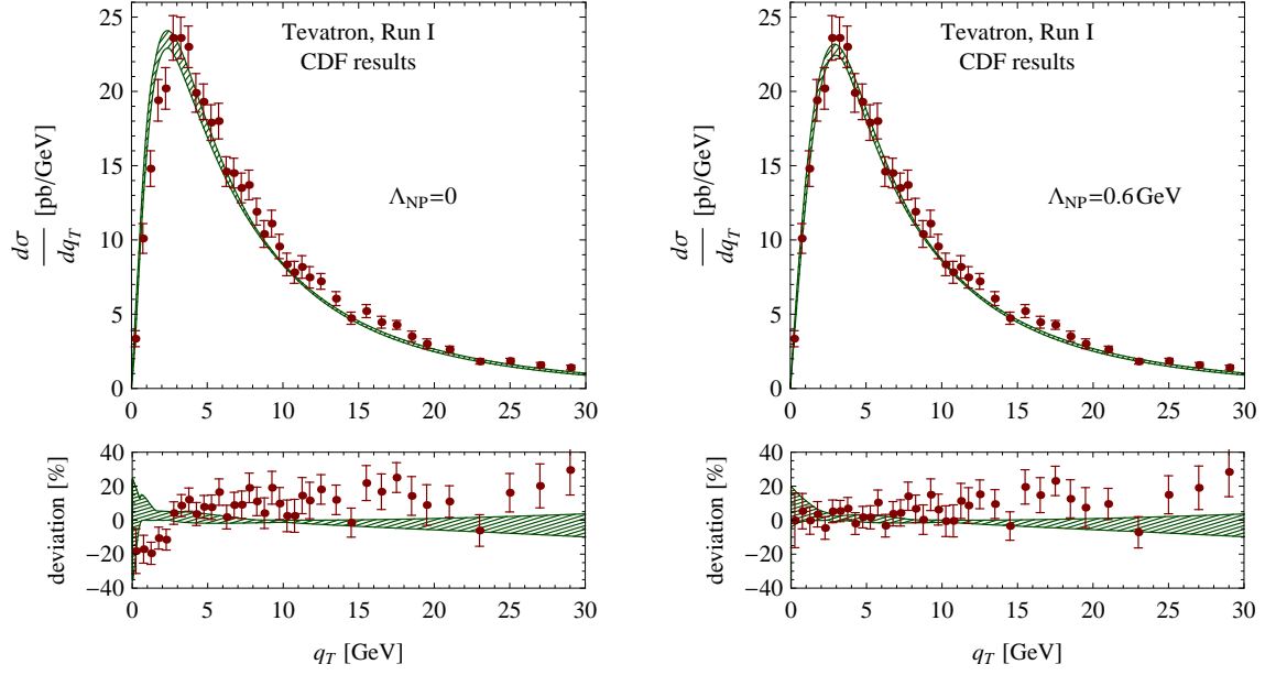
Figure 7.2. Comparison with Tevatron Run I data from CDF, with and without long-distance corrections, taken from [50]. The lower panels show the deviation from the default theoretical prediction.
