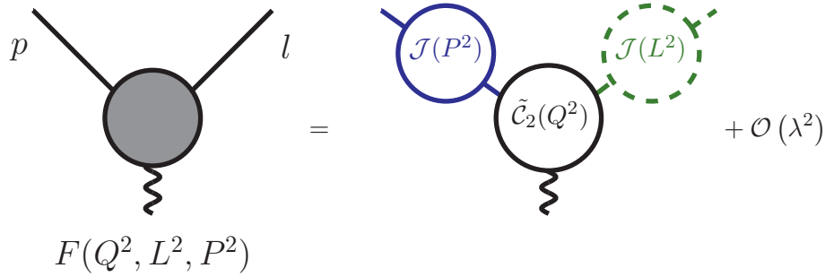
Figure 3.3. Diagrammatic representation of the factorization theorem for the \phi^3 theory in d = 6 .
