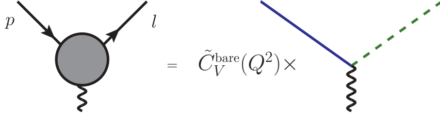
Figure 5.1. Matching condition which allows to obtain \tilde{C}_V^{\text{bare}}(Q^2) . In the calculation of the form factor one should set from the start p^2 = l^2 = 0 .
