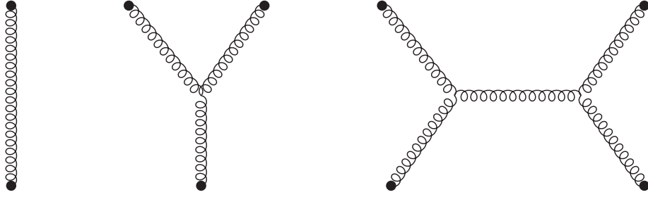
Figure 8.6. The single connected web involving two, three, and four particles. The dots represent color generators, which appear when the gluons are attached to Wilson lines.
