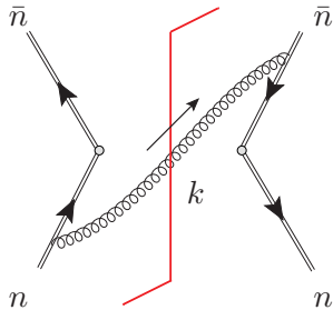
Figure 6.1. One loop Feynman diagram contributing to the soft function. The vertical line (the “cut”) indicates that the gluon crossing it is on-shell.
