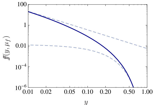
Figure 6.2. Fall-off of the parton luminosity function ff(y, \mu_f) for \mu_f = 8 \text{ GeV} . The dashed lines show the asymptotic behavior for small and large y . Figure taken from [10].
