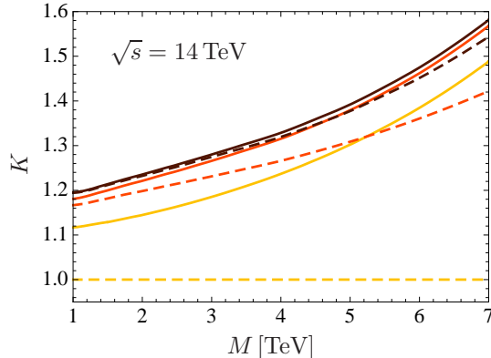
Figure 6.4. Resummed (solid lines) versus fixed-order results (dashed lines) for the K -factor as a function of M . The light, medium, and dark lines correspond to LO, NLO, and NNLO, respectively. Default values are used for all scales.
