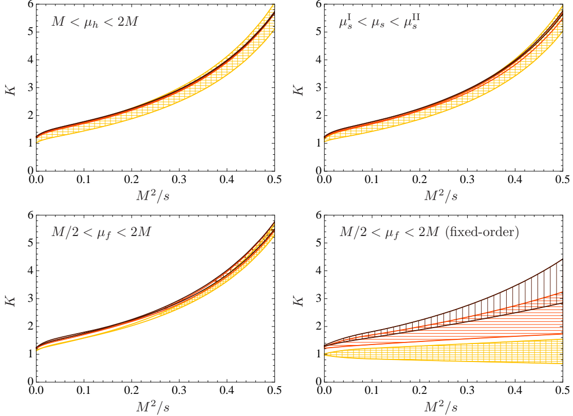
Figure 6.3. Dependence of the resummed Drell-Yan cross section for M = 20 GeV on the scales \mu_h , \mu_s , and \mu_f . The bands show the K -factor obtained at NLL (light), NNLL (medium), and NNNLL (dark). The last plot shows for comparison the \mu_f dependence in fixed-order perturbation theory at LO, NLO, and NNLO.
