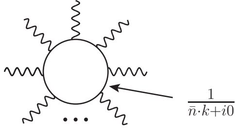
Figure 4.1. Diagrammatic representation of the diagrams corresponding to the determinant originating from the integration over \eta .
