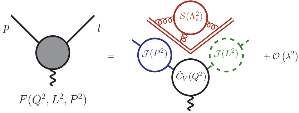
Figure 4.2. Diagrammatic representation of the Sudakov form factor in QCD; the diagram illustrates the separation of the different scales present in the problem. The soft scale is \Lambda_s^2 = L^2 P^2 / Q^2 .
