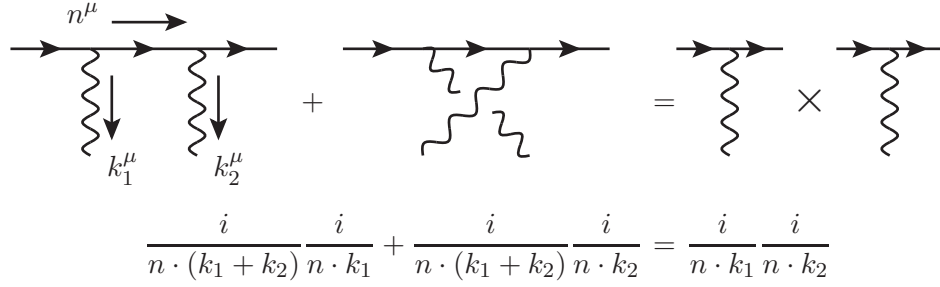
Figure 8.2. Diagrammatic relation between products of eikonal propagators in QED. n^\mu identifies the direction along which the particle emitting soft photons is moving.
