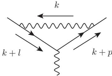
Figure 2.1. One-loop vertex corrections. The Feynman diagram is here shown in terms of fermions and photons, however, the spin structure is neglected in this section.
