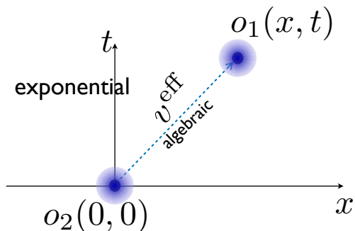
Figure 2.3: Correlations between observables at the Euler scale are due to propagation of ballistic waves between the two observables.
