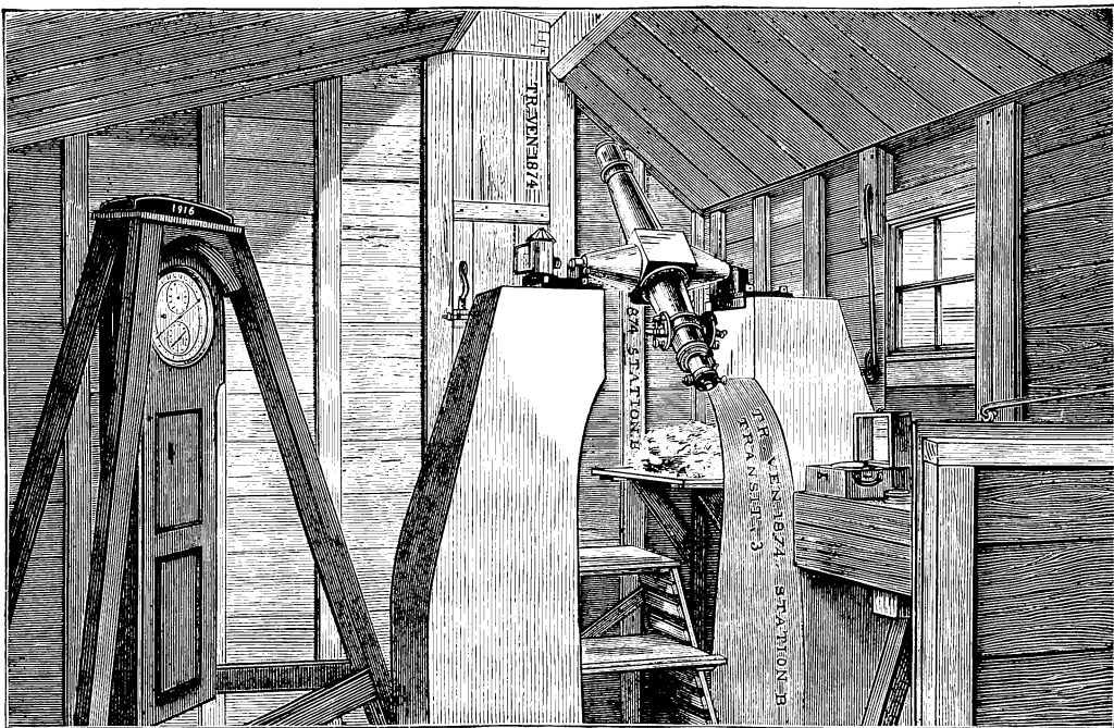
FIG. 76.—A Transit-instrument for the British astronomical expedition, 1874. Shewing in its essential features the simplest form of such an instrument.
