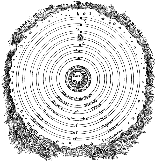
FIG. 8.—Ptolemaic system.
