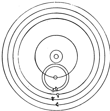
FIG. 11.—Egyptian system.
