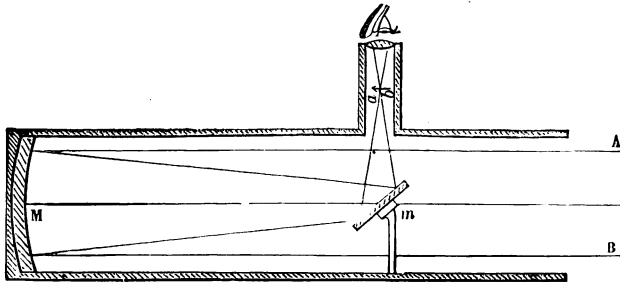
FIG. 82.—Principle of Newtonian reflector.
