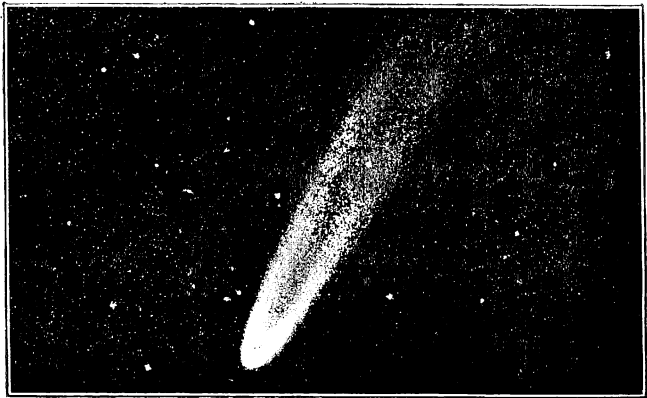
FIG. 102.—Halley's Comet.
