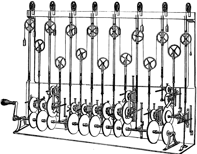
FIG. 119.—Tide-predicter, for combining the ascertained constituents into a tidal curve for the future.
