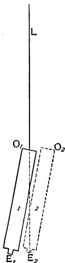
FIG. 78.—Aberration diagram. The light-ray L penetrates the object glass of the moving telescope at O_1 , but does not reach the eyepiece until the telescope has travelled to the second position. Consequently a moving telescope does not point out the true direction of the light, but aims at a point a little in advance.
