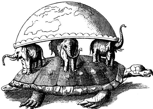
FIG. 6.—Hindoo Earth.
