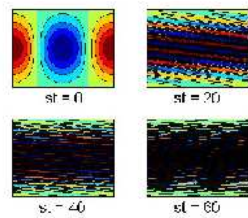
Figure 31: Evolution of \omega(x, y, t) from an initial vorticity perturbation \omega(x, y, 0) = \omega_1(y, 0) \cos(x) , by the linearized 2D Euler equations close to a shear flow U(y) = \sigma y . (colors in the .PDF document)
