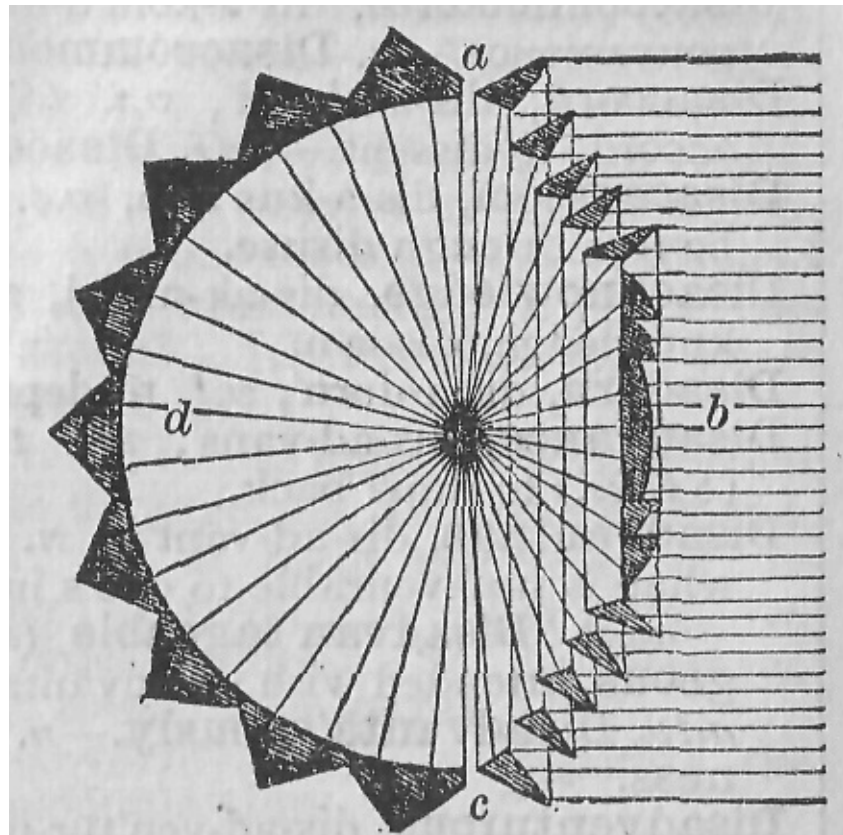
Transverse section of Dioptric System, showing rays of light passing through the dioptric lenses, a , b , c , in parallel lines, assisted by reflection from the dioptric spherical mirror, a , d , c .
