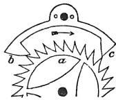
Anchor, or Recoil, Escape-ment : a , escape-wheel ; b , c , pallets.
