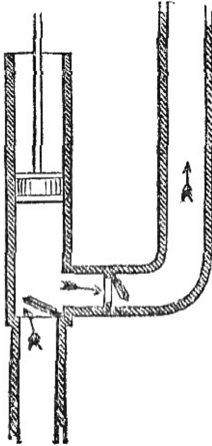
Section of Force-pump.
