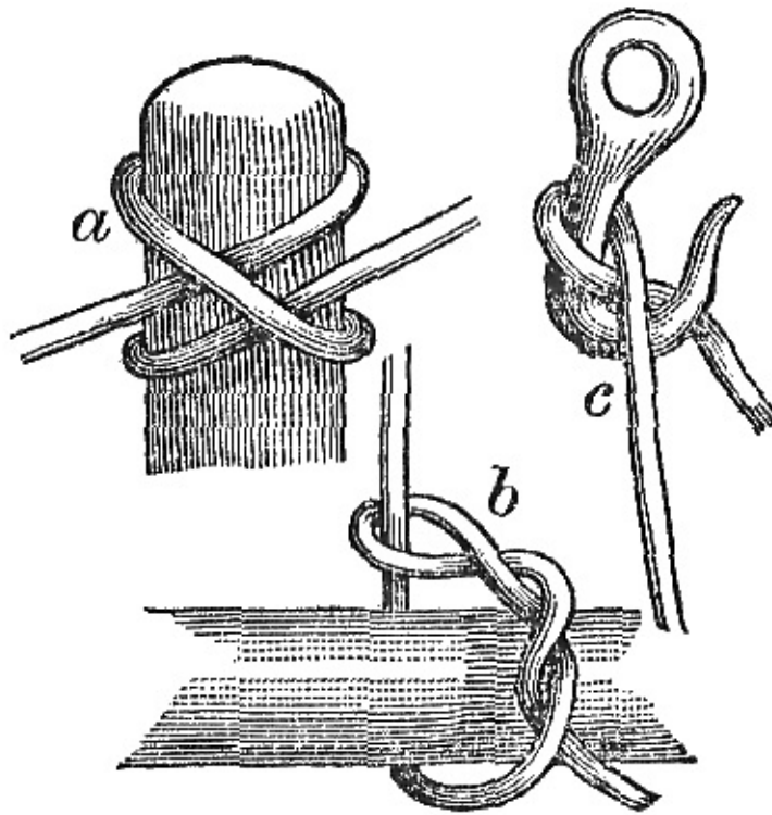
a , Clove-hitch; b , Timber-hitch; c , Blackwall-hitch.
