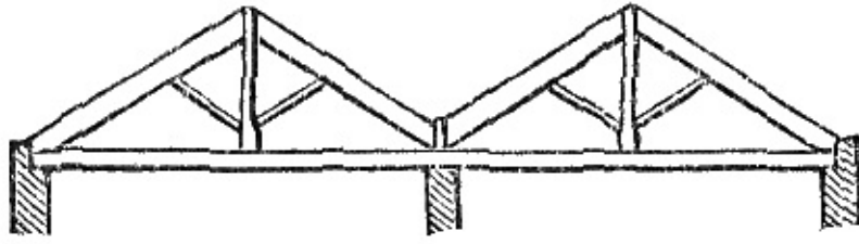
M-roof.
