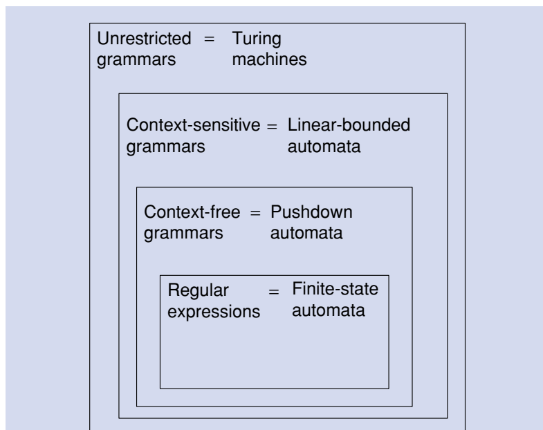
The Chomsky hierarchy with computational equivalent
