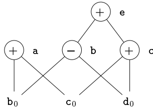
Figure 8.13: DAG for basic block in Example 8.11
