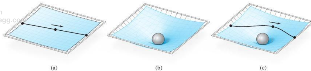
figure 7.7.7 (a) A particle on a taut trampoline moves in a straight line. (b) A heavy steel ball distorts the trampoline. (c) A particle on the distorted trampoline follows a curved path.
