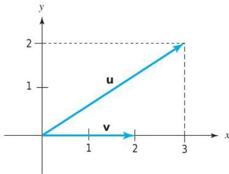
figure 1.1.11 Find \mathbf{u} + \mathbf{v} and -2\mathbf{u} .
