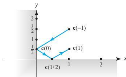
figure 4.2.2 A piecewise smooth path.
