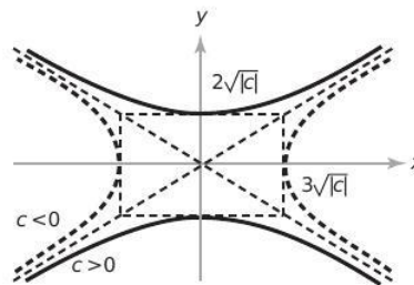
Level curves
