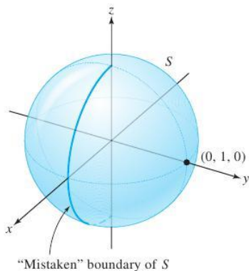
figure 8.2.3 The surface S is a portion of a sphere.
