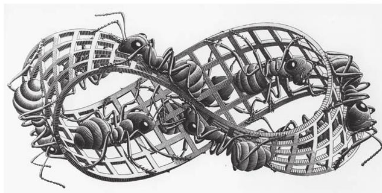
figure 7.6.4 Ants walking on a Möbius strip.
