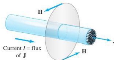
figure 8.2.15 Ampère's law.
