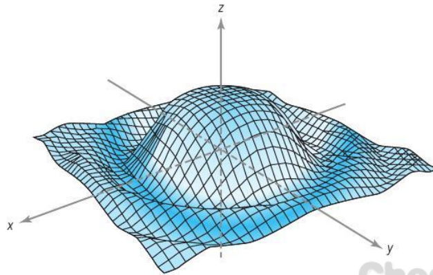
figure 2.2.17 Graph of the function f(x, y) = \frac{\sin(x^2 + y^2)}{x^2 + y^2} .
