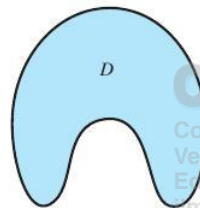
figure 8.1.10 Prove Green's theorem for this region.
