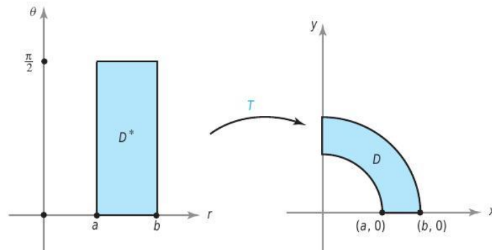
figure 6.2.8 The polar coordinate mapping takes a rectangle D^* onto part of an annulus D .
