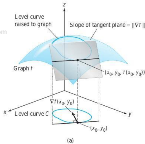
figure 2.R.1 (a) The relationship between the gradient of a function and the tangent plane to the graph (Exercise 23(a)). For a specific instance of the tangent plane in (b) see Exercise 23(b).
