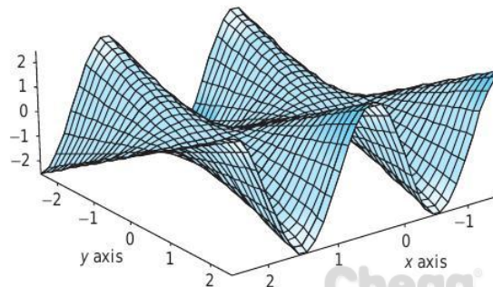
figure 3.R.3 Graph of z = y \sin(\pi x) .
