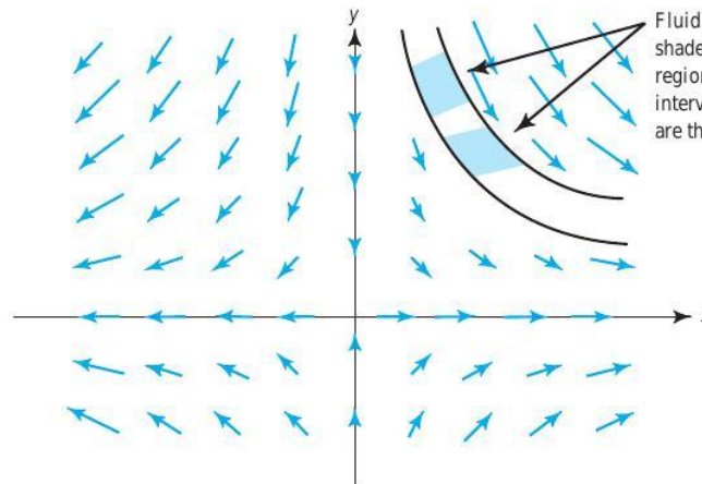
figure 4.4.6 The vector field \mathbf{F}(x, y) = x\mathbf{i} - y\mathbf{j} . ▲
