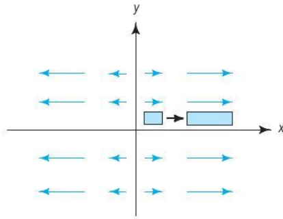
figure 4.4.2 This fluid is expanding.
