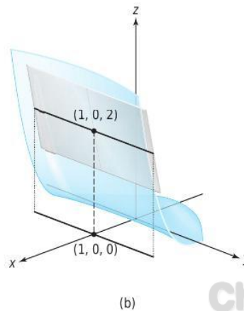
figure 2.R.1 (a) The relationship between the gradient of a function and the tangent plane to the graph (Exercise 23(a)). For a specific instance of the tangent plane in (b) see Exercise 23(b).
