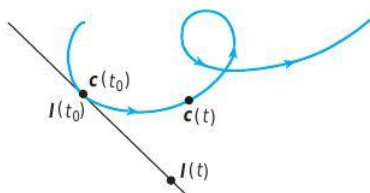
figure 2.4.11 The tangent line to a path.
