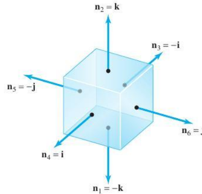
figure 8.4.3 The outward orientation on the cube.
