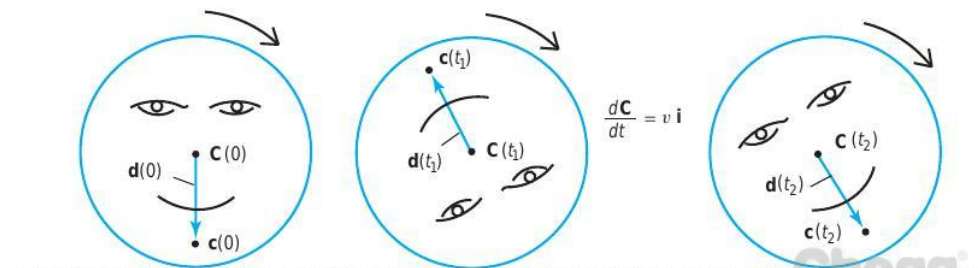
figure 2.4.5 The vector \mathbf{d}(t) points from the wheel's center, \mathbf{C}(t) , to the position \mathbf{c}(t) of a point on the wheel and rotates in the clockwise direction while the wheel moves to the right.
