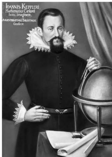
figure 10 Johannes Kepler (1571–1630).
