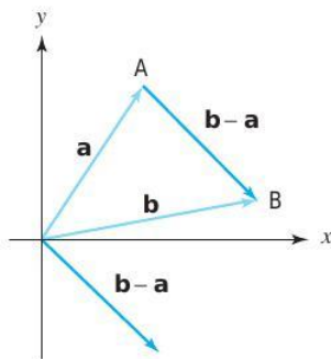
figure 1.1.10 The geometry of vector subtraction.
