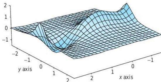
figure 3.R.1 Graph of z = (3x^4 - 4x^3 - 12x^2 + 18)/12(1 + 4y^2) .
