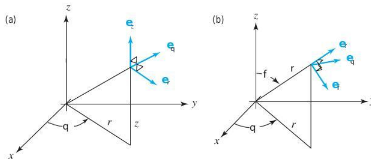
figure 1.4.8 (a) Orthonormal vectors \mathbf{e}_r, \mathbf{e}_\theta, and \mathbf{e}_z associated with cylindrical coordinates. The vector \mathbf{e}_r is parallel to the line labeled r . (b) Orthonormal vectors \mathbf{e}_\rho, \mathbf{e}_\theta, and \mathbf{e}_\phi associated with spherical coordinates.
