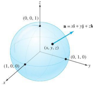
figure 8.4.6 \mathbf{n} is the unit normal to \partial W , the boundary of the ball W . Copyright © W. H. Freeman Vector Calculus Edition: 6 jimmybo2@gmail.com Printed from www.chegg.com
