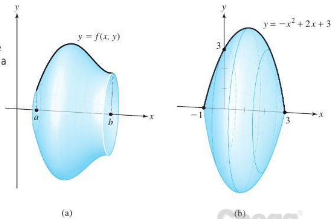
figure 5.1.13 The solid of revolution (a) has volume \pi \int_a^b (f(x))^2 dx .
