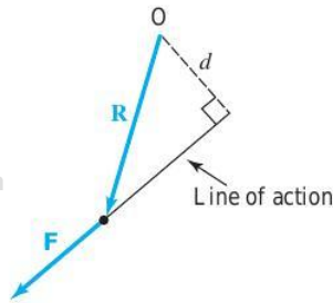
figure 1.3.10 Moment of a force.
