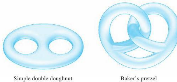
figure 7.7.11 Two manifestations of a surface S in R³ of genus 2.
