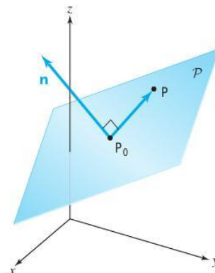
figure 1.3.6 The points P of the plane through P_0 and perpendicular to \mathbf{n} satisfy the equation \vec{P_0P} \cdot \mathbf{n} = 0 .
