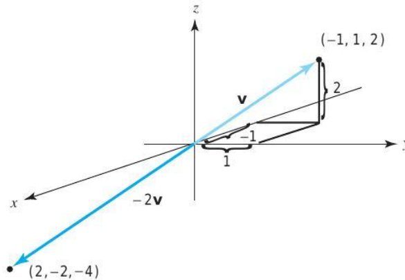
figure 1.1.13 Multiplying (-1, 1, 2) by -2 .
