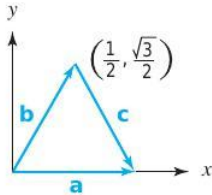
figure 1.2.3 The vectors a , b , and c are represented by the sides of an equilateral triangle.
