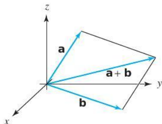
figure 1.1.5 The geometry of vector addition.
