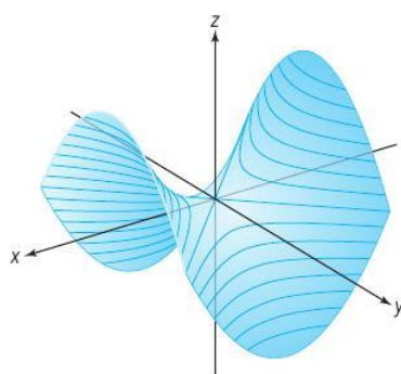
figure 2.1.11 The graph of z = x^2 - y^2 and its level curves.
