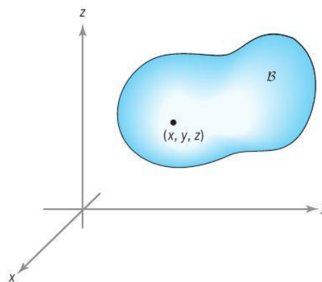
figure 3.1.2 A homogeneous body in space.
