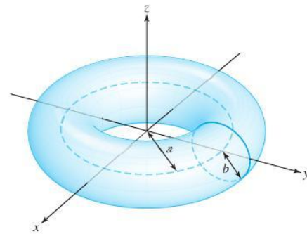
figure 8.4.10 The surface for Exercise 30(c).
