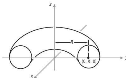
figure 7.4.6 A cross section of a torus.
