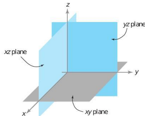
figure 1.1.26 The three coordinate planes.
