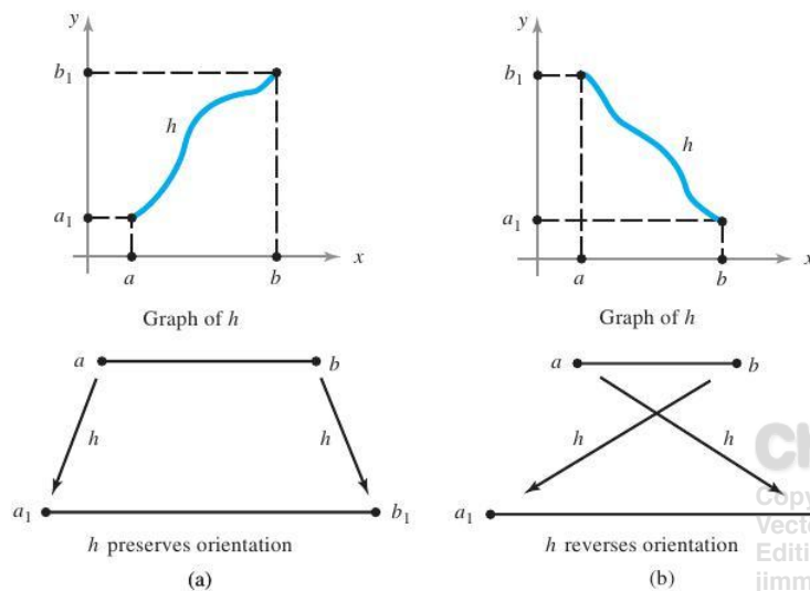
figure 7.2.4 Illustrating (a) an orientation-preserving reparametrization, and (b) an orientation-reversing reparametrization.
