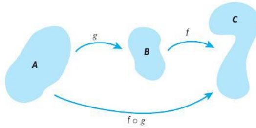
figure 2.2.15 The composition of f on g .
