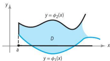
figure 6.4.5 An unbounded region D .
