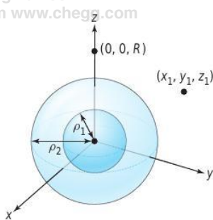
figure 6.3.5 The gravitational potential at (x_1, y_1, z_1) is the same as at (0, 0, R) , where R = \sqrt{x_1^2 + y_1^2 + z_1^2} .
