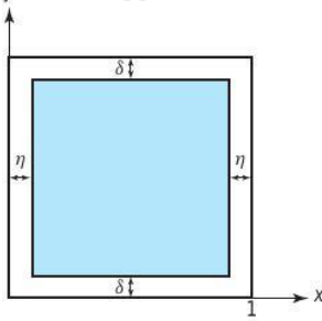
figure 6.4.3 The slightly shrunken unit square.
