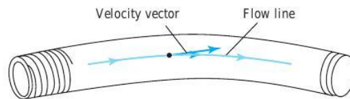
figure 4.3.8 The velocity vector of a fluid is tangent to a flow line.
