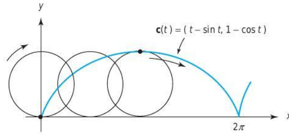
figure 2.4.6 The curve traced by a point moving on the rim of a rolling circle is called a cycloid.
