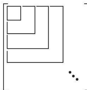
figure 3.3.5 “Diagonal” submatrices are used in the criterion for positive definiteness; they must all have determinant > 0 .
