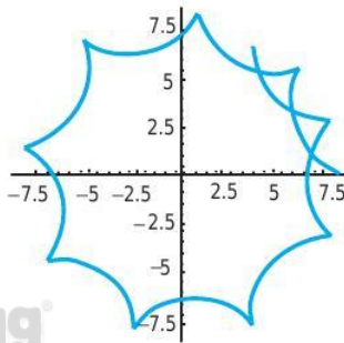
figure 2.4.7 An example of a hypocycloid.
