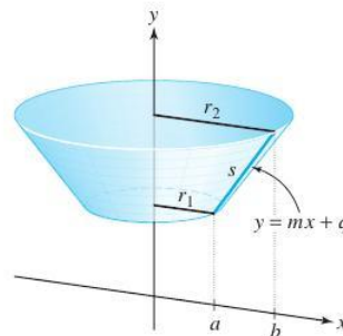
figure 7.4.7 A line segment revolved around the y axis becomes a frustum of a cone.
