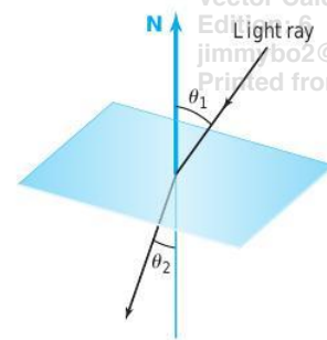
figure 1.3.11 Snell's law.
