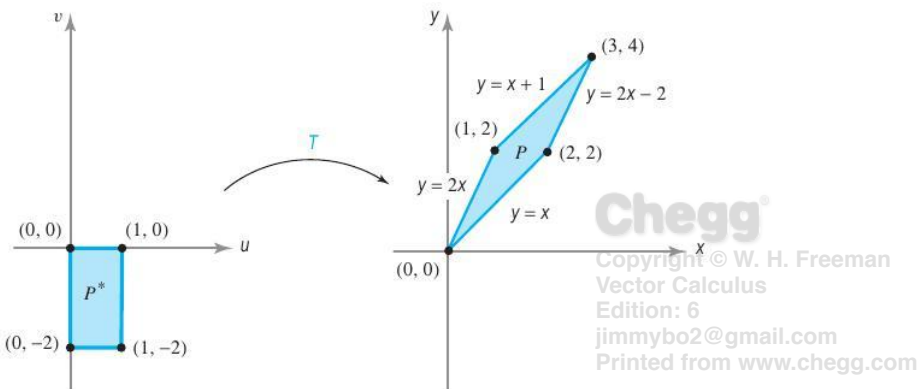
figure 6.2.6 The effect of T(u, v) = (u - v, 2u - v) on the rectangle P^* .
