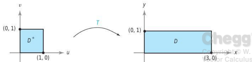
figure 6.2.1 The map T: (u, v) \mapsto (-u^2 + 4u, v) takes the square D^* onto the rectangle D .
