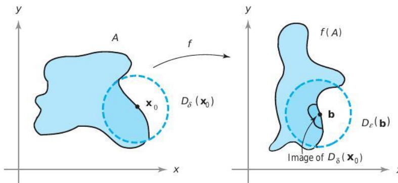
figure 2.2.16 The geometry of the \epsilon - \delta definition of limit.
