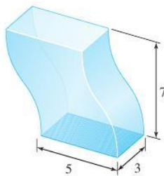
figure 5.1.11 Compute this volume.
