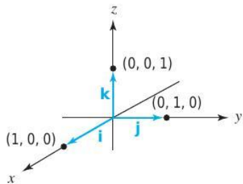
figure 1.1.14 The standard basis vectors.
