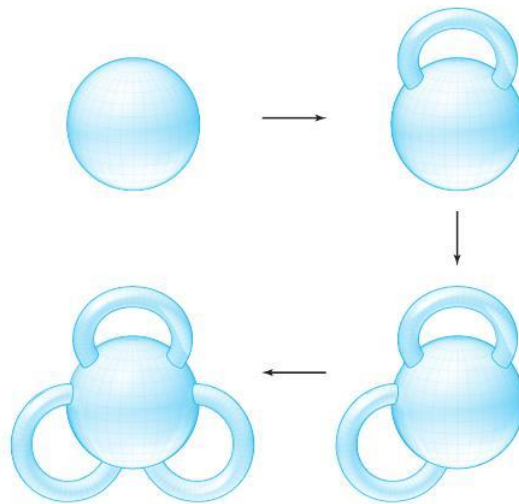
figure 7.7.10 A sphere with 0, 1, 2, 3 handles attached.
