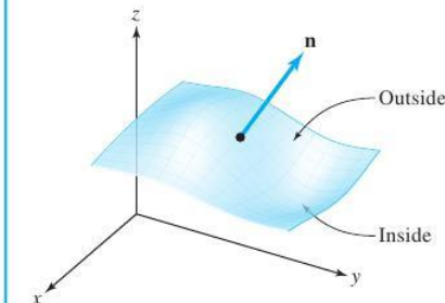
figure 7.6.6 \mathbf{n} points away from the outside of the surface.
