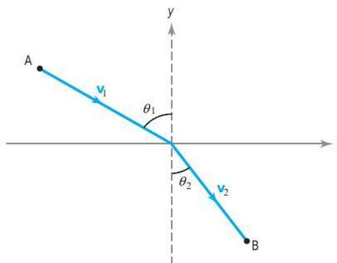
figure 3.4.7 Snell's law of refraction.
