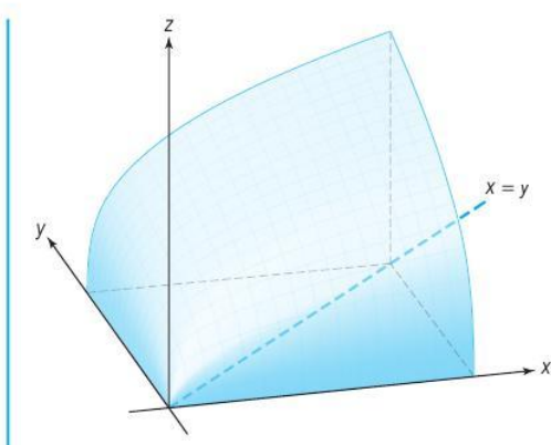
figure 2.3.2 The portion of the graph of x^{1/3}y^{1/3} in the first quadrant.
