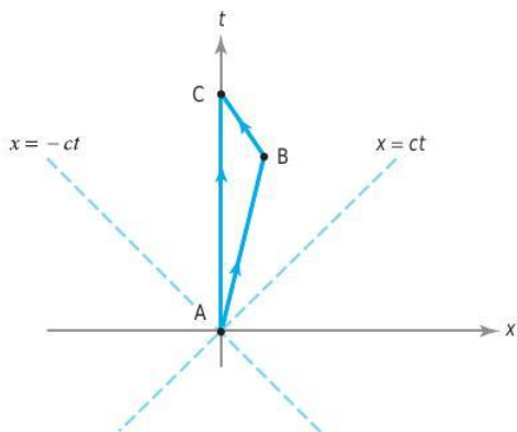
figure 4.2.6 The relativistic triangle inequality.
