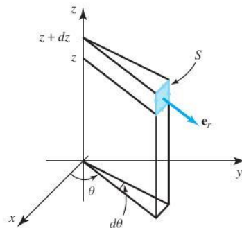
figure 8.2.9 A surface element in cylindrical coordinates.
