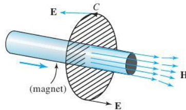
figure 8.2.11 Faraday's law.
