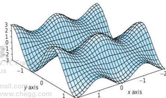
figure 3.R.2 Graph of z = (2 + \cos \pi x)(\sin \pi y) .
