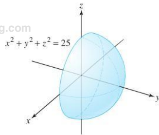
figure 8.4.9 The surface for Exercise 30.
