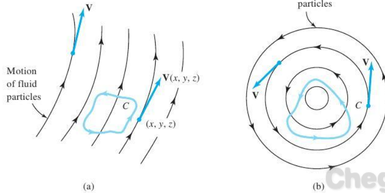
figure 8.2.7 Circulation of a vector field (velocity field of a fluid): (a) Circulation about C is zero; (b) nonzero circulation about C ("whirlpool").
