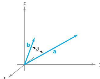
figure 1.2.1 \theta is the angle between the vectors \mathbf{a} and \mathbf{b} .
