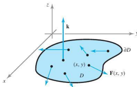
figure 8.1.7 The vector form of Green's theorem.
