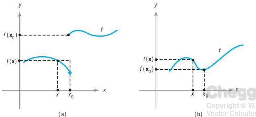
figure 2.2.13 (a) Discontinuous function for which \lim_{x \rightarrow x_0} f(x) does not exist. (b) Continuous function for which this limit exists and equals f(x_0) .
