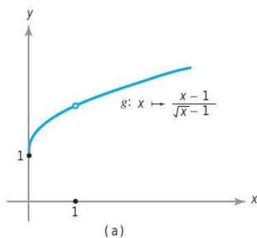
figure 2.2.11 These graphs are the same except that in part (a), g is undefined at x = 1 , whereas in part (b), g^* is defined for all x \geq 0 .
