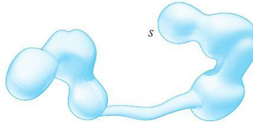
figure 7.7.8 A deformed sphere. \frac{1}{2\pi} \iint_S K \, dA = 2.
