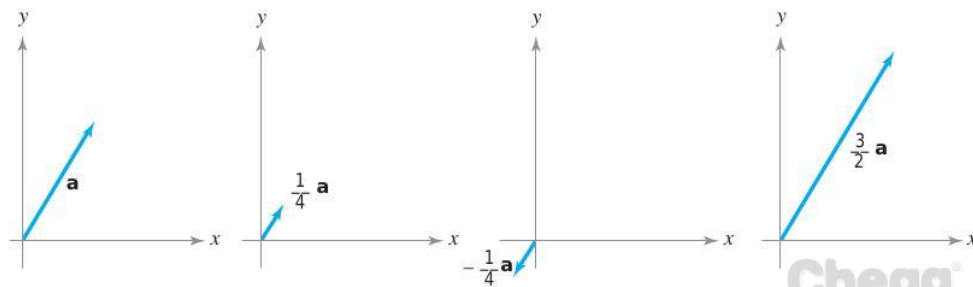
figure 1.1.9 Some scalar multiples of a vector \mathbf{a} .
