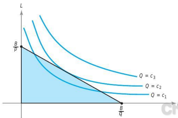
figure 3.4.5 What is the largest value of Q in the shaded triangle?
