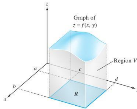
figure 5.1.1 The region V in space is bounded by the graph of f , the rectangle R , and the four vertical sides indicated.
