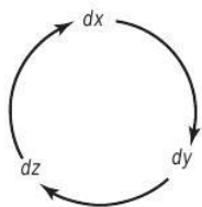
figure 8.5.1 The cyclic order of dx , dy , and dz .
