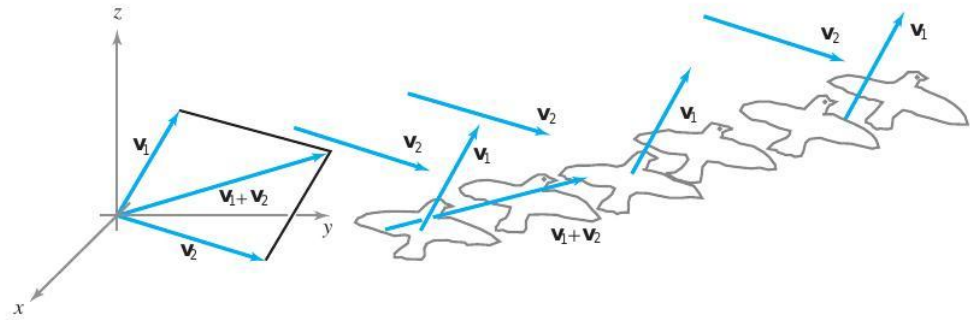
figure 1.1.6 A physical interpretation of vector addition.
