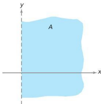
figure 2.2.4 Show that A is an open set.
