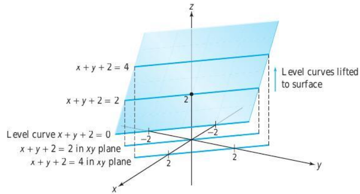
figure 2.1.5 The relationship of level curves of Figure 2.1.4 to the graph of the function f(x, y) = x + y + 2 , which is the plane z = x + y + 2 .
