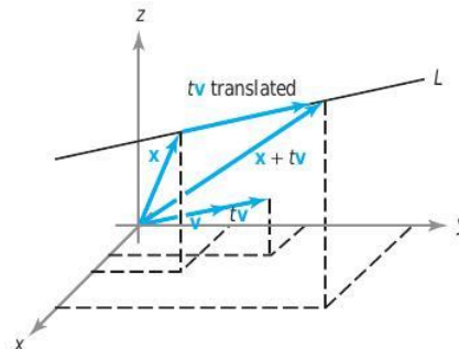
figure 2.6.1 The equation of L is \mathbf{l}(t) = \mathbf{x} + t\mathbf{v} .
