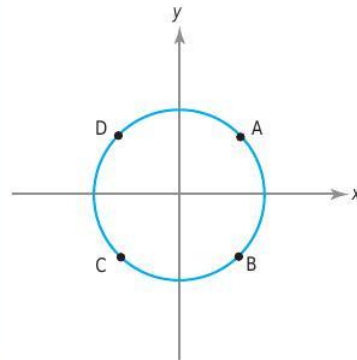
figure 3.4.6 The four critical points in Example 11.
