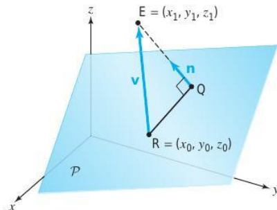
figure 1.3.7 The geometry for determining the distance from the point E to plane \mathcal{P} .
