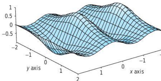
figure 3.R.4 Graph of z = \sin(\pi x)/(1 + y^2) .
