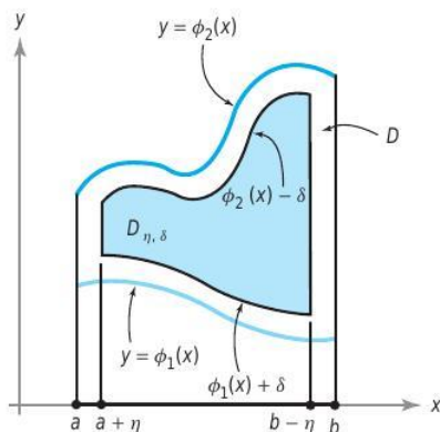
figure 6.4.2 A shrunk domain D_{\eta, \delta} for improper integrals.
