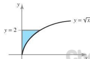
figure 5.R.1 The region of integration for Exercise 16.
