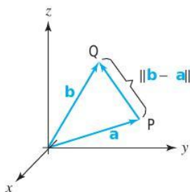
figure 1.2.5 The distance between the tips of a and b is \|\mathbf{b} - \mathbf{a}\| .
