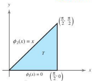
figure 5.3.6 A triangle T represented as a y -simple region.
