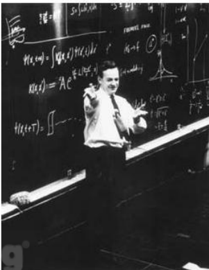
figure 4.1.6 Feynman lecturing at Caltech.
