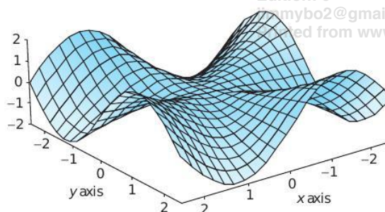
figure 3.1.4 The graph of the function in Exercise 32.
