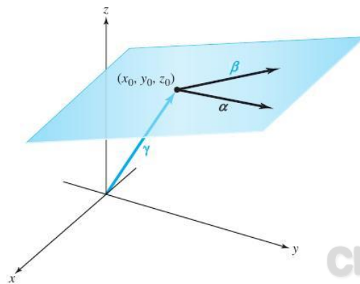
figure 7.3.6 Describing a plane parametrically.
