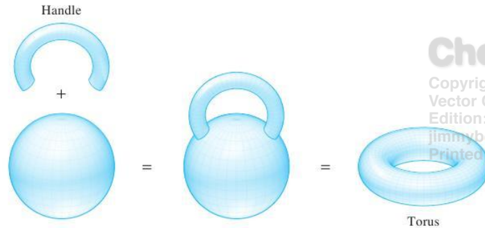
figure 7.7.9 Gluing a handle to a sphere to obtain a torus.
