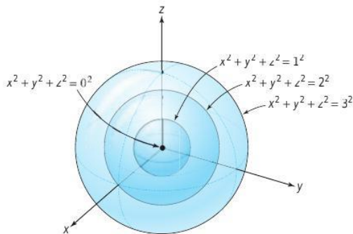
figure 2.1.12 Some level surfaces for f(x, y, z) = x^2 + y^2 + z^2 .
