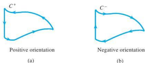
figure 8.1.1 (a) Positive orientation of C , and (b) negative orientation of C .
