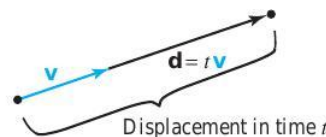
figure 1.2.17 Displacement = time \times velocity.
