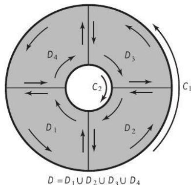
figure 8.1.5 Green's theorem applies to D = D_1 \cup D_2 \cup D_3 \cup D_4 .
