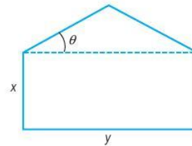
figure 3.3.8 Maximize the area for fixed perimeter.
