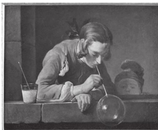
figure 7.4.5 A boy blowing a soap bubble. Painting by the French artist Jean Baptiste Siméon Chardin (1699–1779). The Metropolitan Museum of Art, New York.
