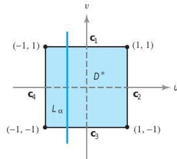
figure 6.1.3 Domain for the transformation T of Example 2.
