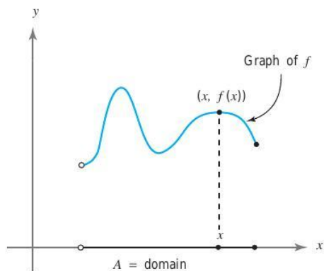
figure P.3 The graph of a function with the half-open interval A as domain.
