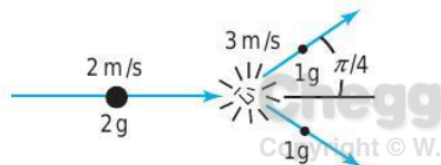
figure 1.R.1 Momentum and marbles.
