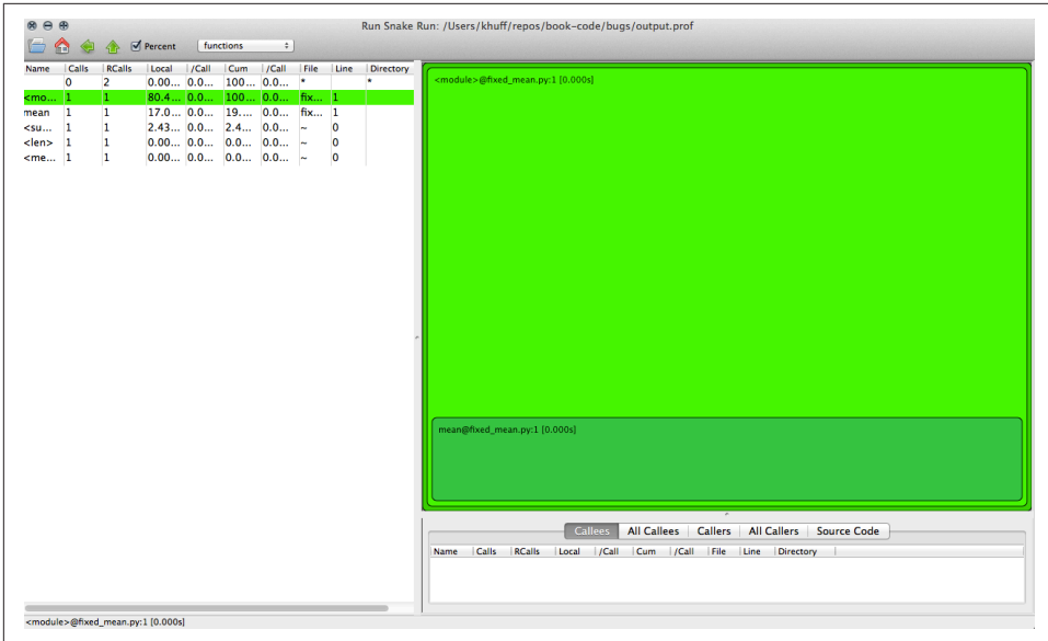
Figure 17-1. Profiling the mean function with RunSnakeRun
