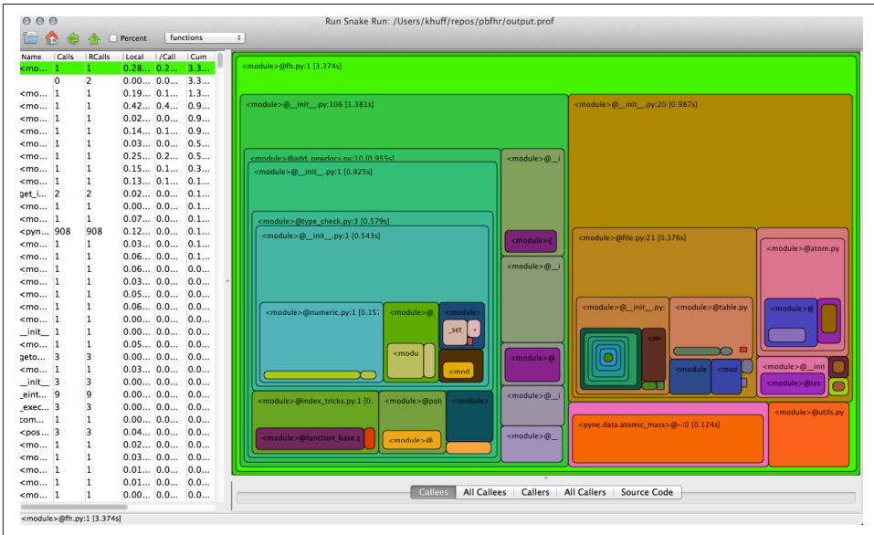
Figure 17-2. Profiling a more complex script with RunSnakeRun
